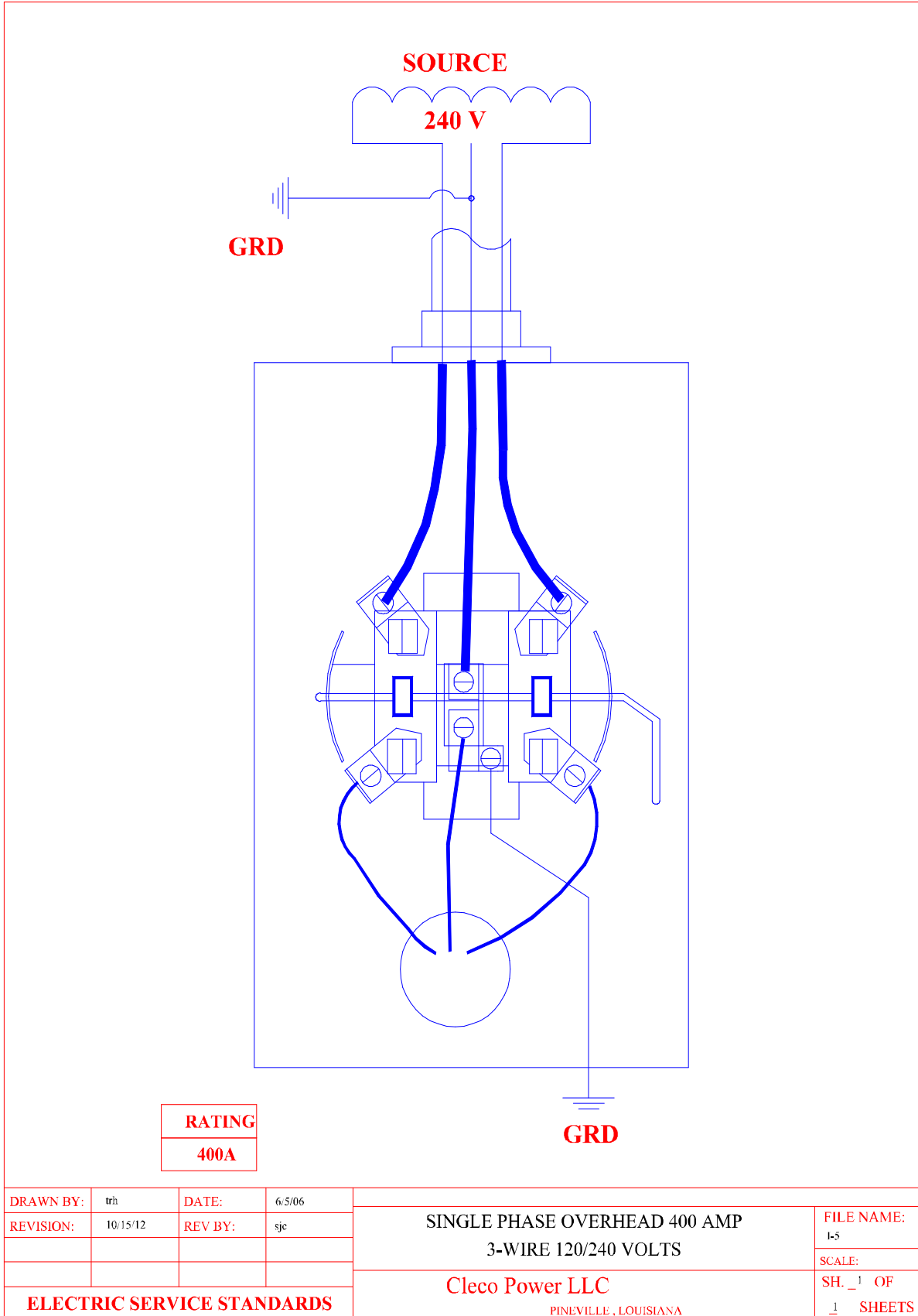
Fig. I-5 Single-Phase OH 400A 3-Wire 120/240 Volts
