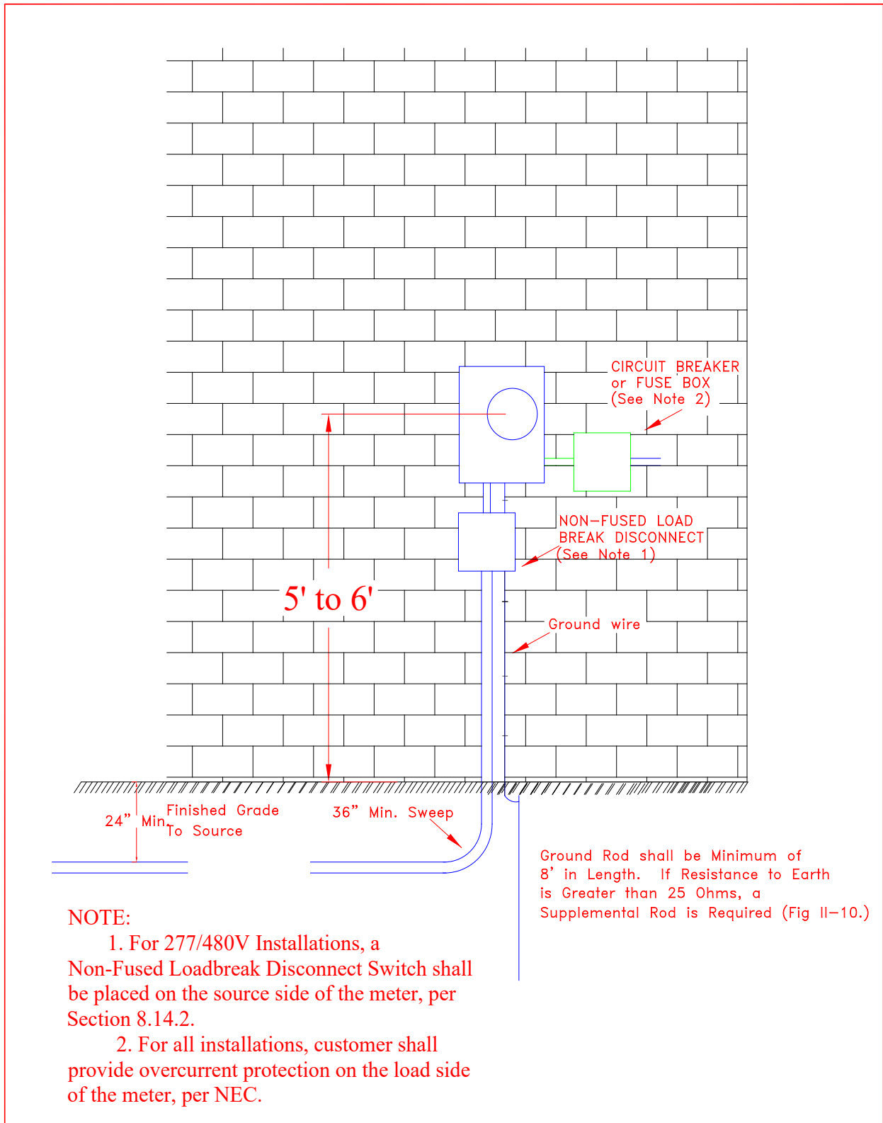
Fig. III-13 Padmount Transformer site Details
