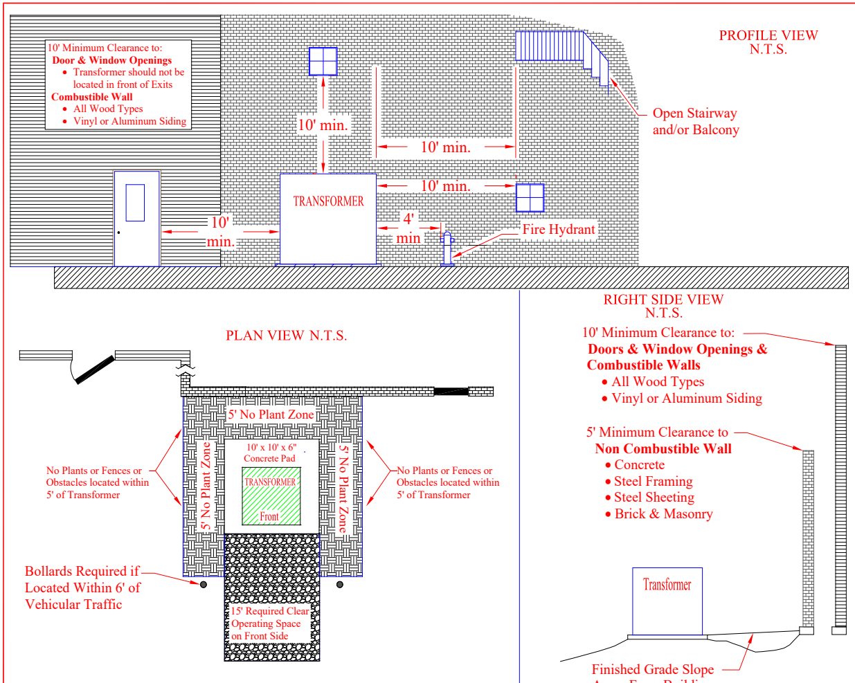
Fig. III-12 URD Temporary Service
