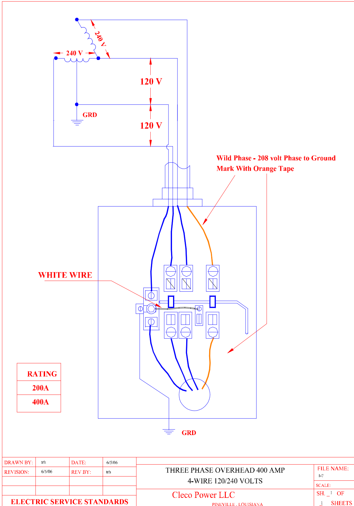
Fig. I-7 Three-Phase 120/240 Volts
