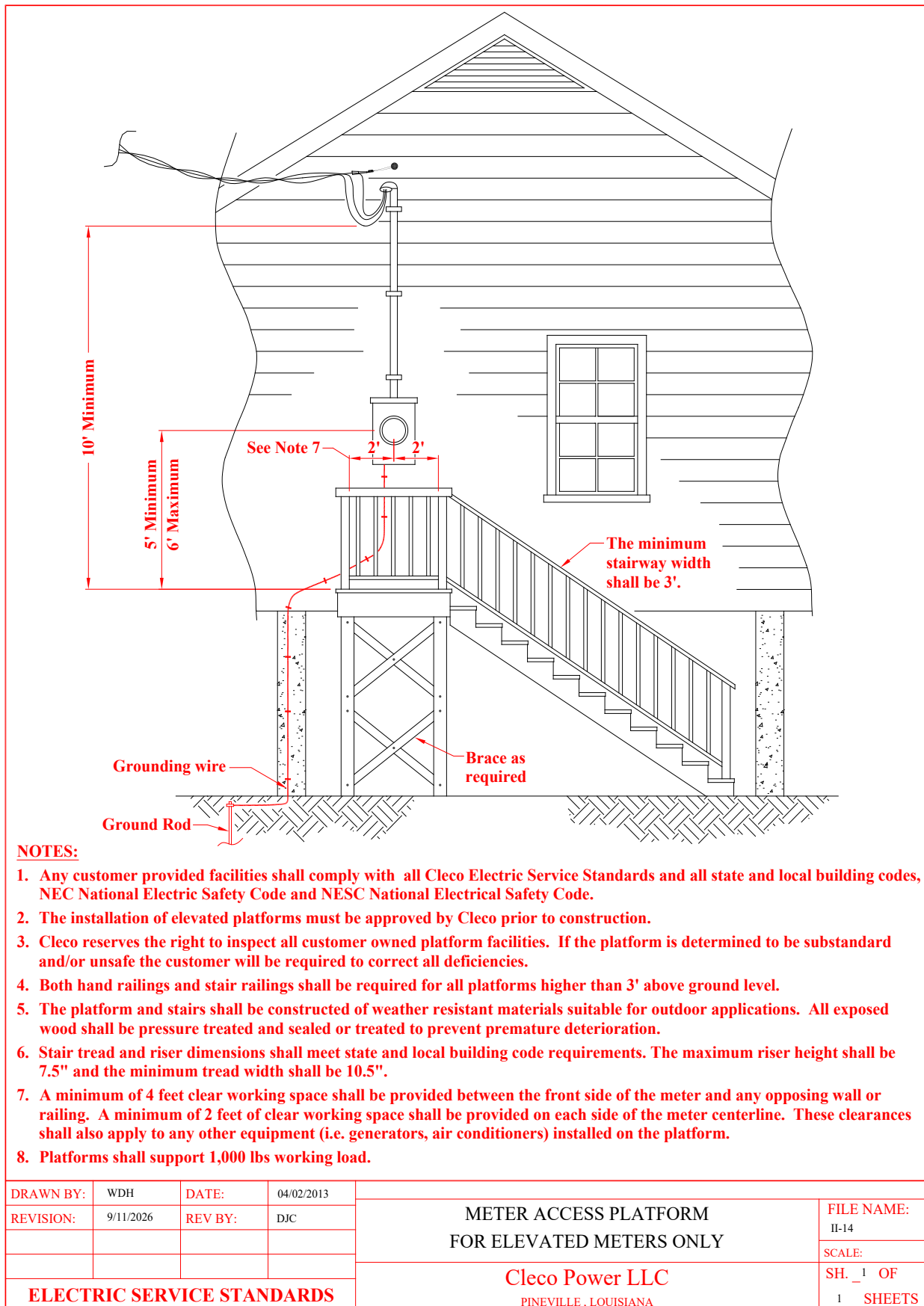
Fig. II-14 Meter Access Platform for Elevated Meters Only
